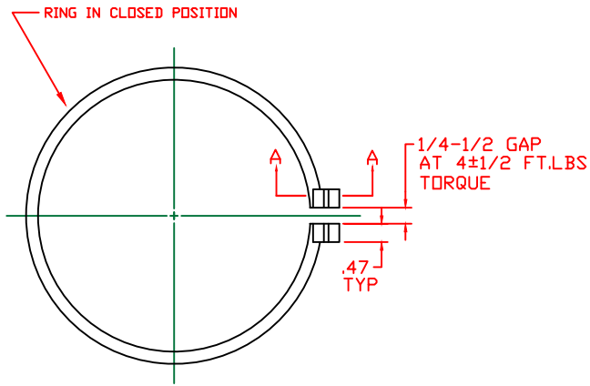
LOCKING RING
