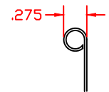
CURL DETAIL
