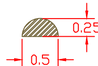
ALT. GASKET MS27683 -100 THRU -106
