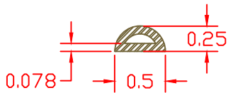
GASKET MS27683 -90 THRU -96
