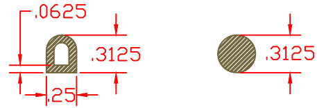
GASKET MS27684-25
