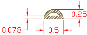
GASKET MS27683 -90 THRU -96
