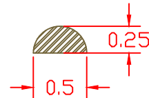
ALT. GASKET MS27683 -100 THRU -106
