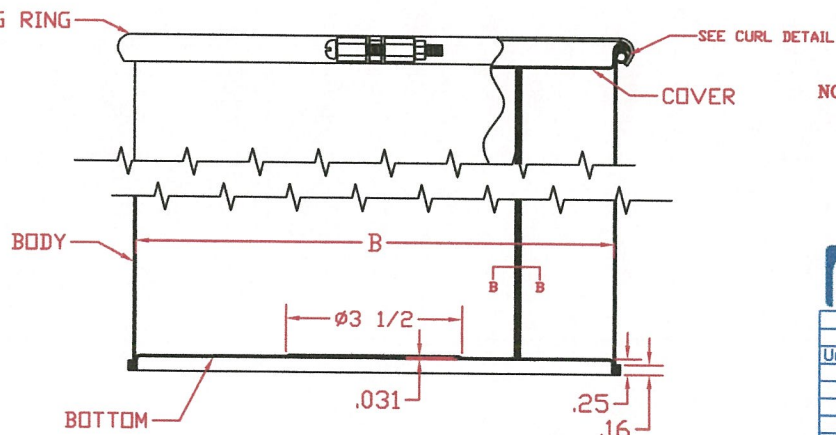
LOCKING RING
