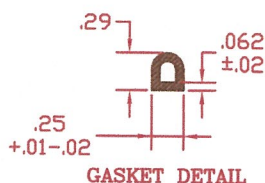
GASKET DETAIL
