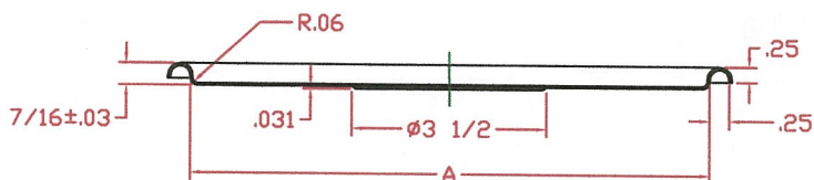
LOCKING RING
