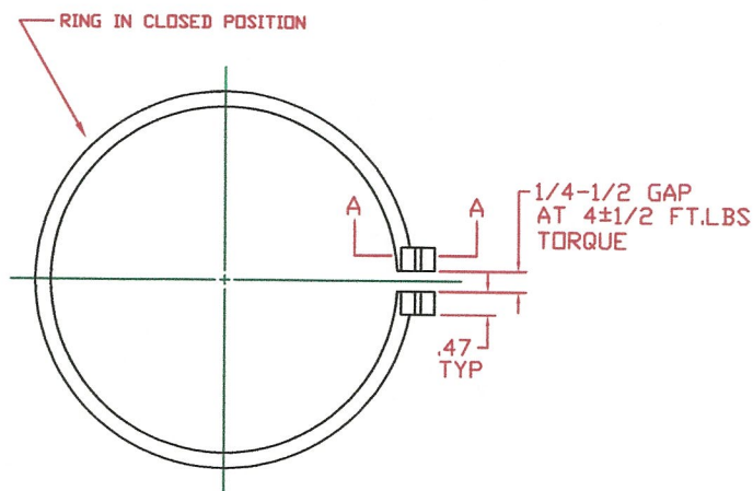
LOCKING RING
